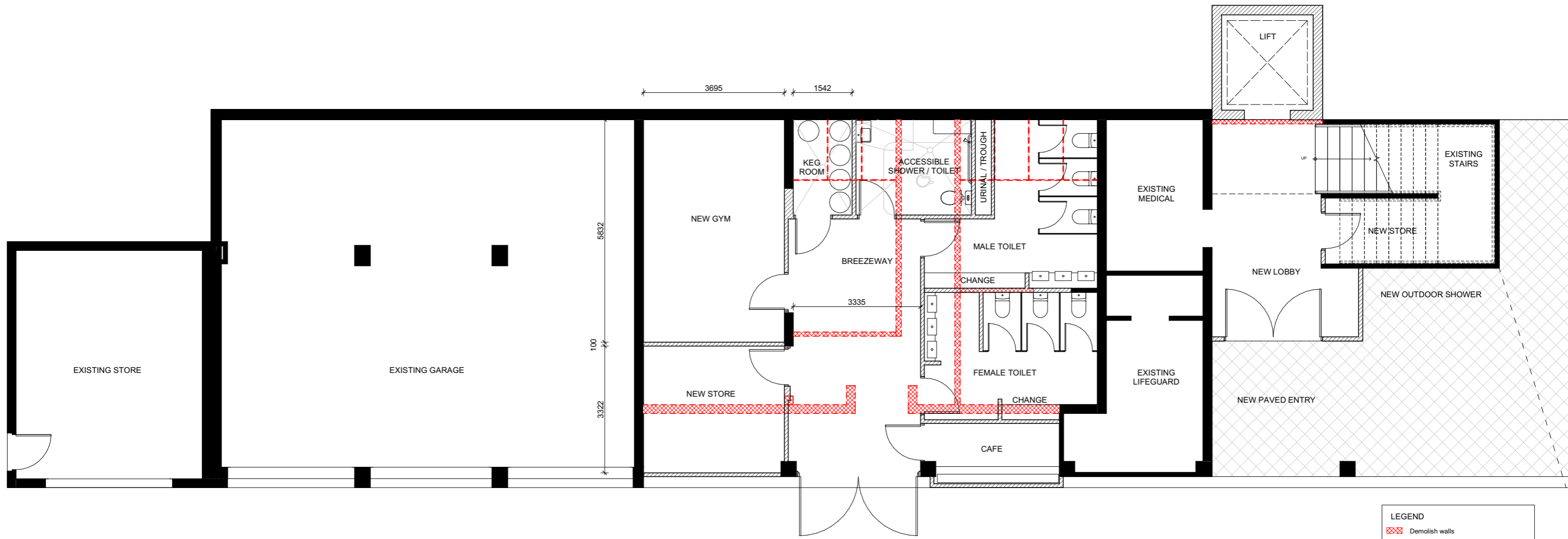
1 GROUND FLOOR PLAN SCALE 1:50
